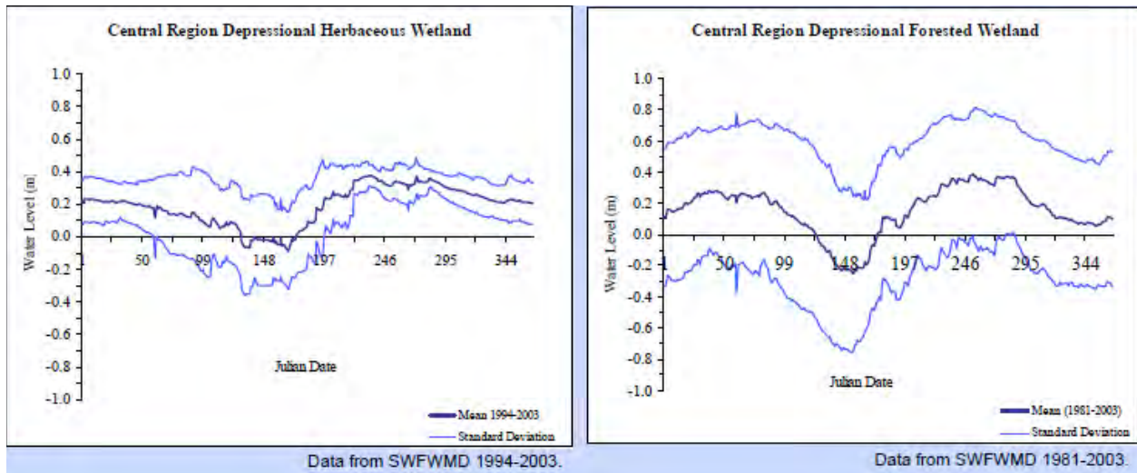
Figure B-1. Figure from Bardi et al. (2005), data compiled from the Southwest Florida Water Management District (SWFWMD) from 1994-2003 for a reference standard central Florida depressional herbaceous wetland (left) and 1981-2003 for a reference standard central Florida depressional forested wetland (right).
