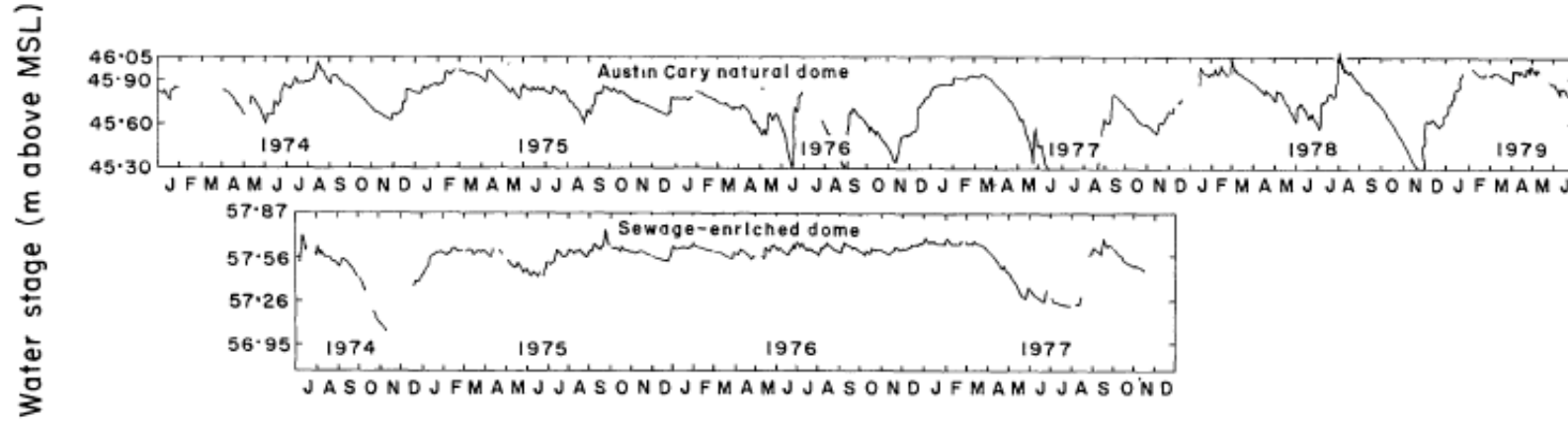
Figure B-13. Figure 1 from Dierberg and Brezonik (1983). Austin Cary natural dome (top) is a reference standard wetland; Sewage-enriched dome (bottom) is an impacted wetland. Original caption reads: “Water level fluctuations in the surface water at the centres of Austin Cary natural (1974-1979) and sewage-enriched (1974-1977) domes. Data collected by K. Heimburg.”
