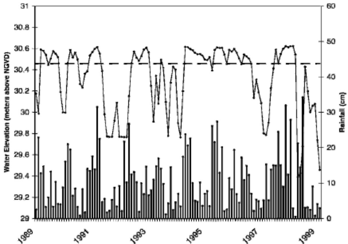
Figure B-4. Figure 2 from Carr et al. (2006). Original caption reads: “Water surface elevation (points and solid line) for median water surface elevation (dashed line) for cypress dome G1 in Lake County, Florida from May 1989 through April 1999. Mean monthly rainfall totals (bars) for 55 stations in Pasco County, Florida are also shown.”
