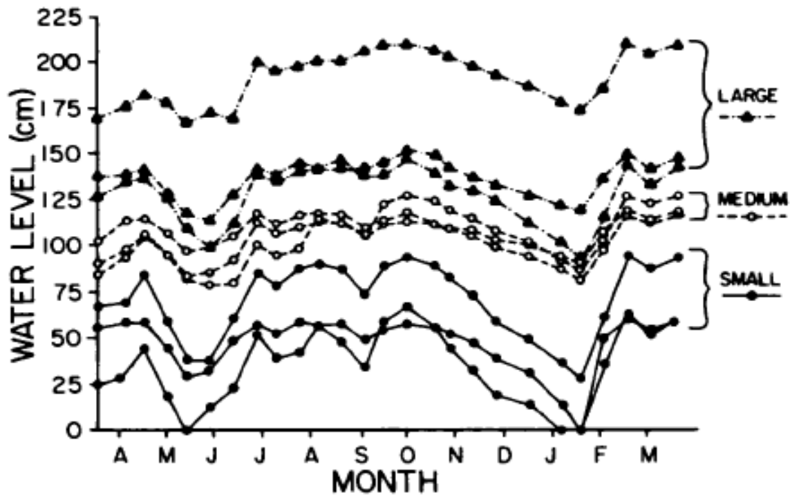
Figure B-15. Figure 5 from Ewel (1990). Original Caption reads: "Typical hydrographs recorded in the centers of nine swamps in central Florida (Ewel and Wickenheiser 1988). Water levels and depths of water above ground in each basin. Small swamps are less than 1 ha, medium swamps are 1-2 ha, and large swamps are more than 5 ha." Taken from Ewel and Wickenheiser (1988), caption: "Biweekly changes in water level (March 1982-March 1983) in the nine study sites."
