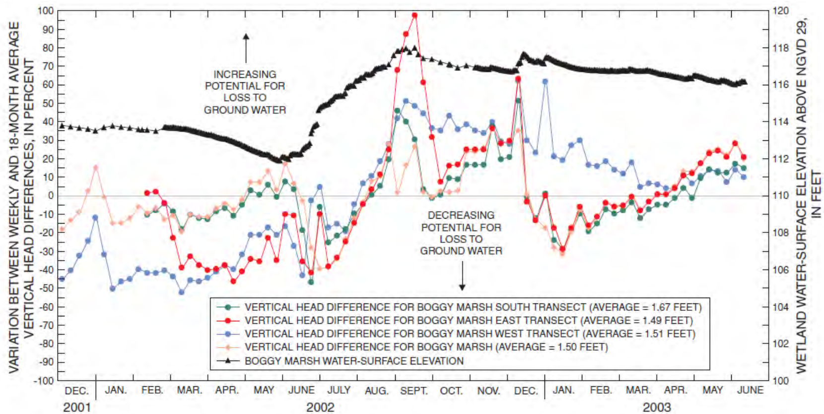
Figure B-19. Figure 32 from Knowles et al. (2005). Original caption reads: “Potential for exchange (vertical) between ground water and Boggy Marsh, Hilochee Wildlife Management Area.”
