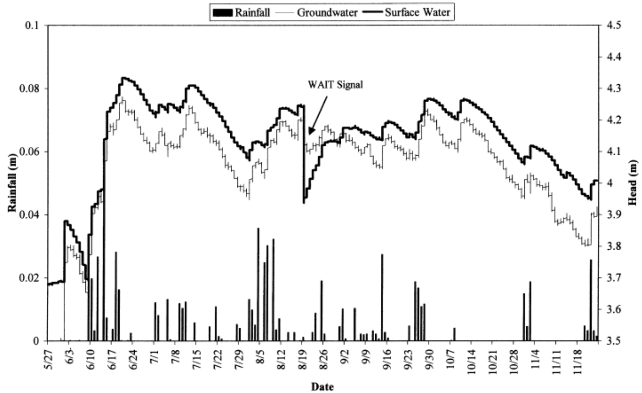
Figure B-24. Figure 3 from Wise et al. (2000). Original caption reads: “Long-term monitoring data including study period.”
