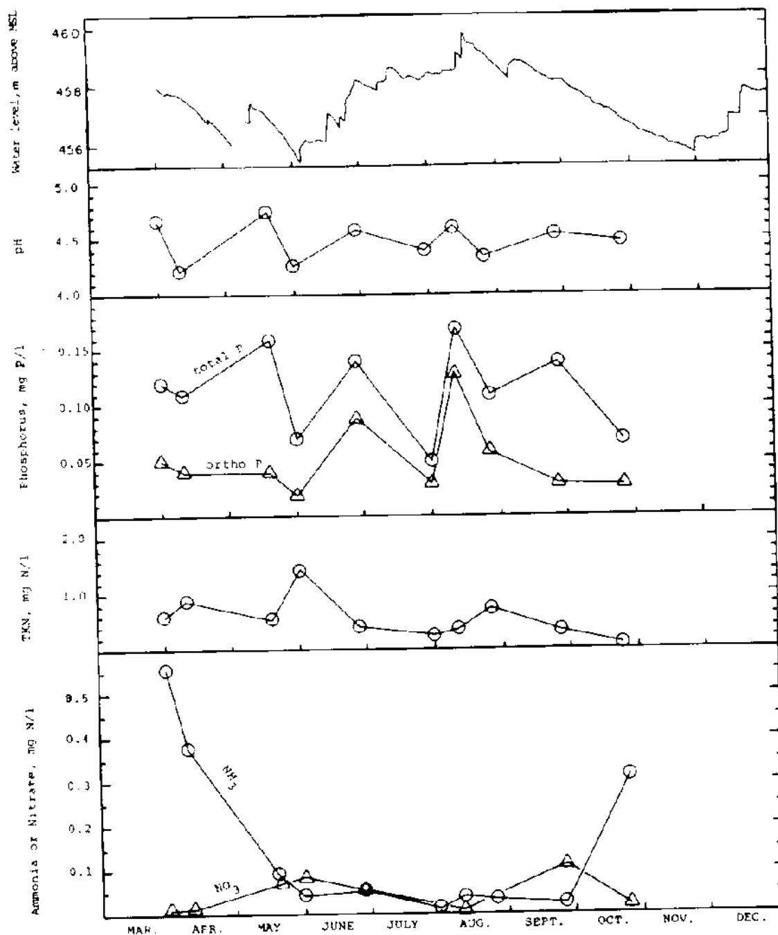
Figure B-20. Figure 3.1 from Mitsch (1984). Original caption reads: "Annual pattern of water level, pH, phosphorus, and nitrogen in the Austin Cary cypress dome pond."
