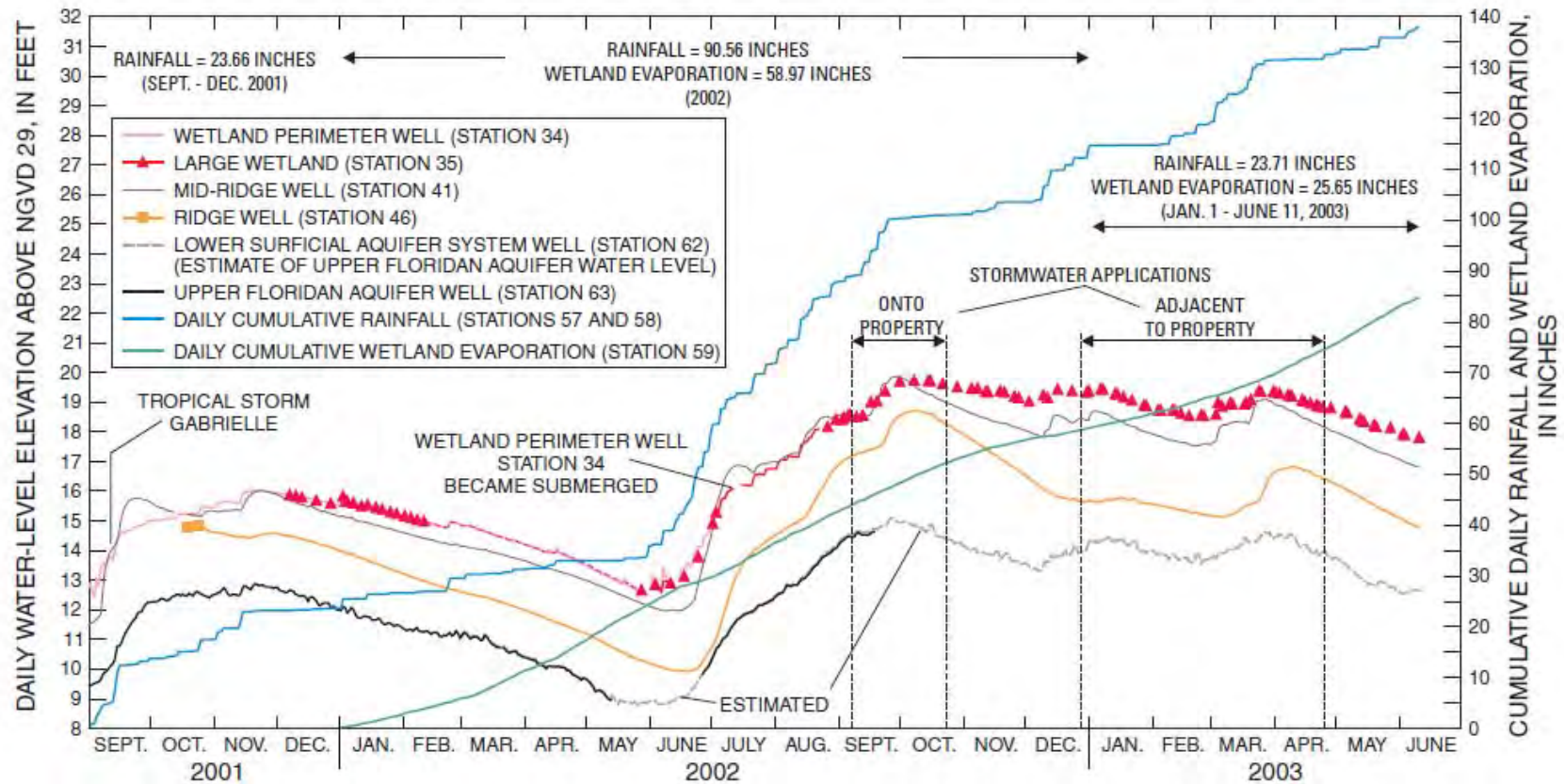
Figure B-18. Figure 20 from Knowles et al. (2005). Original caption reads: “Daily water levels, cumulative rainfall, and cumulative wetland evaporation for the large wetland, Lyonia Preserve (station numbers refer to figure 6 and table 1).”
