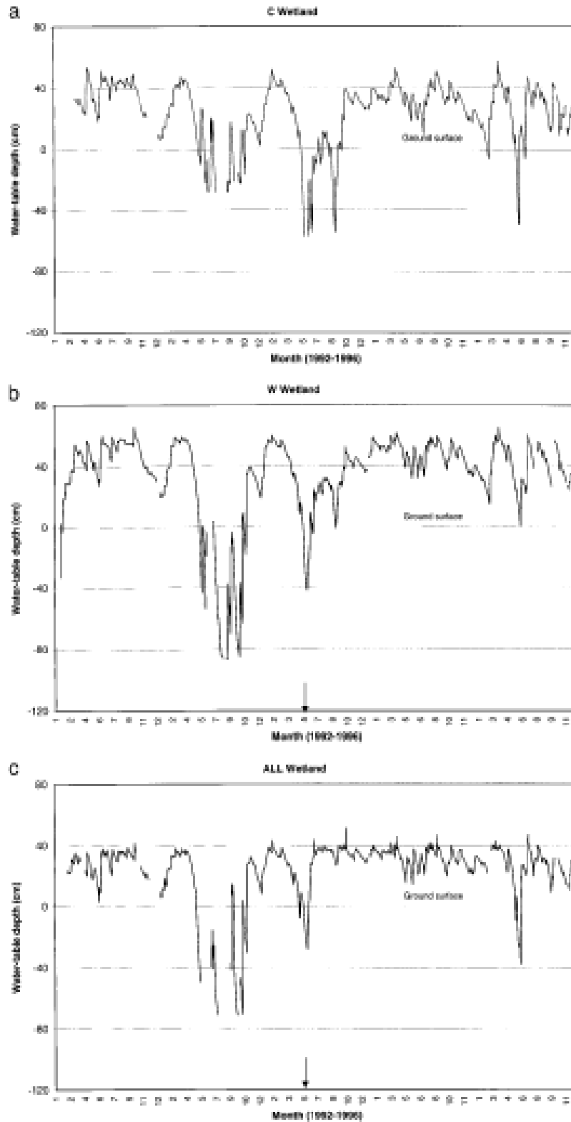
Figure B-23. Figure 1 from Sun et al. (2000). Original caption reads: “Daily water-level dynamics in three cypress wetlands during 1992-1996; the arrow indicates harvesting treatment completed.”
