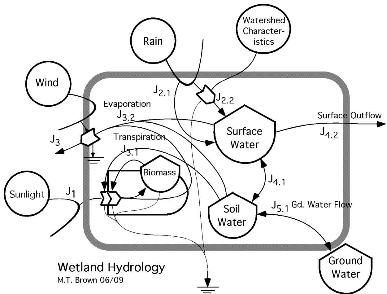
Figure C-1. Wetland Hydrology Model.
