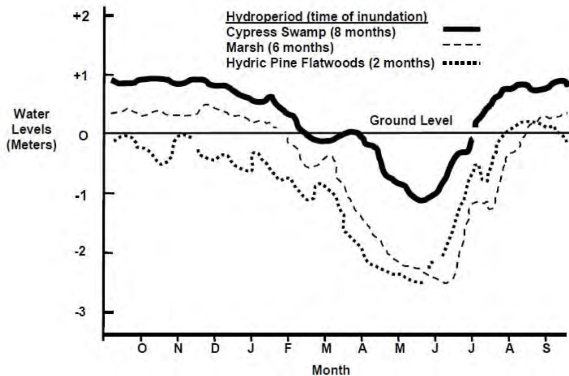
Figure B-14. Figure 7-6 from LWCWSP, summarized from Duever et al. (1986). Original caption reads: "Hydrographs and hydroperiod ranges for three different south Florida vegetation types (Duever et al., 1986)."
