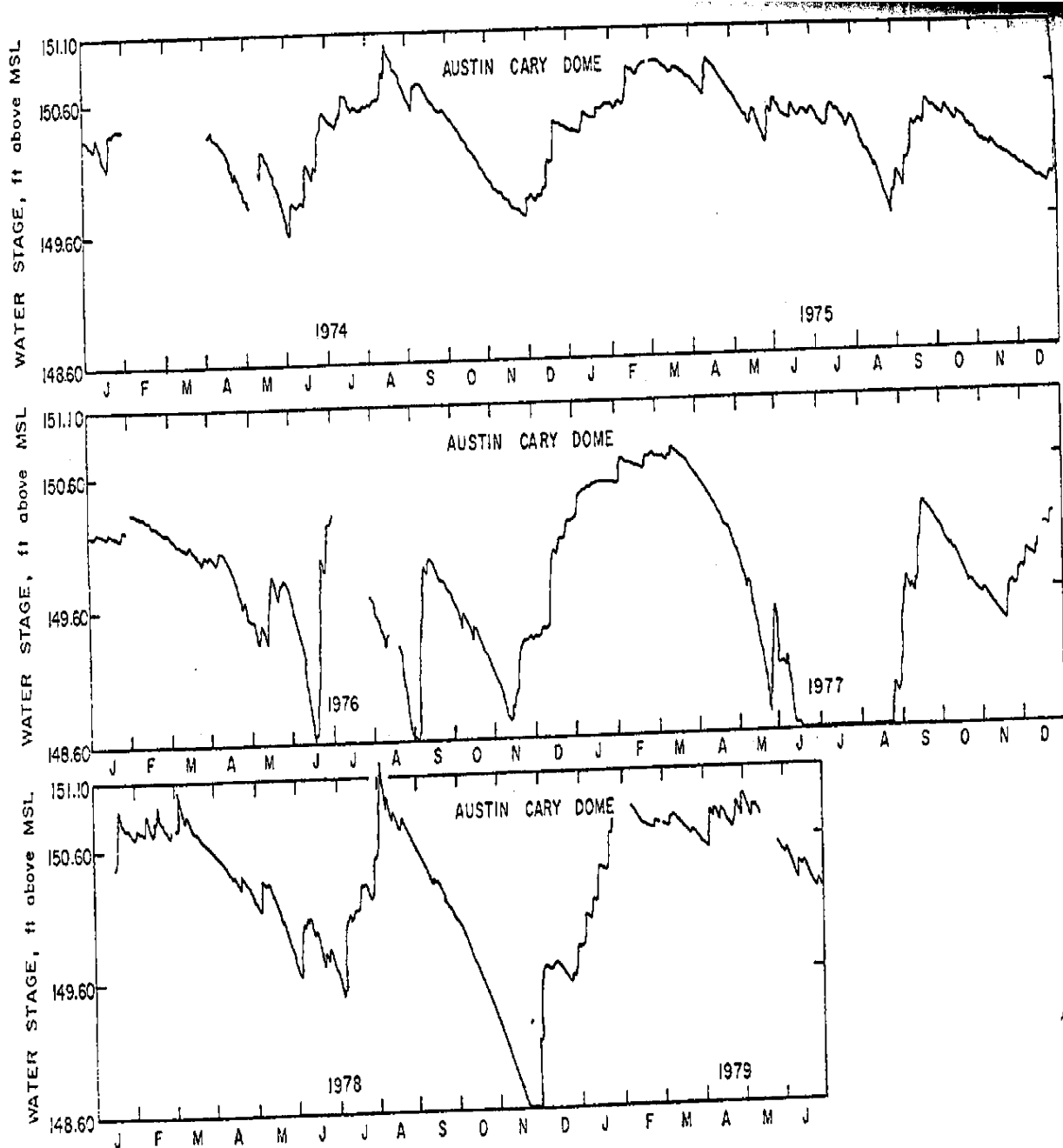
Figure B-12. Figure 7-6 from Dierberg (1980). Original caption reads: "Water level fluctuations in the surface waters of the center of Austin Cary natural dome from 1974 to 1979."
