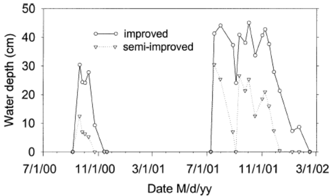
Figure B-22. Figure 1 from Steinman et al. (2003). Original caption reads: “Mean water depth in wetlands from improved and semi-native pastures revealing the seasonal nature of these systems. Data presented in this paper correspond only to the July through October 2001 period.”
