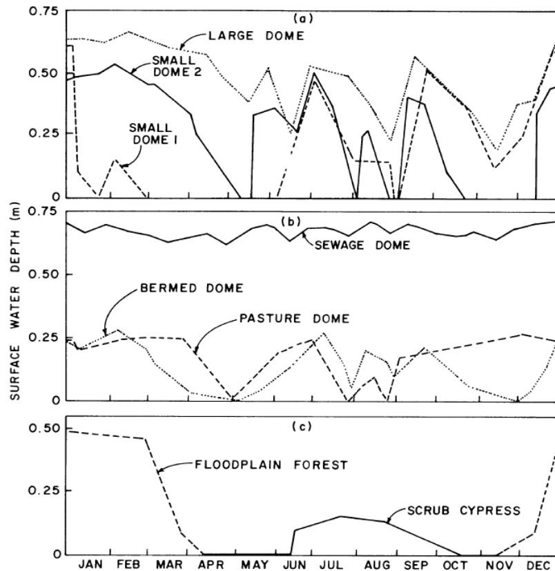
Figure B-3. Figure 2 from Brown (1981). The Large Dome in (a) is considered a reference standard depressional forested wetland. Small Dome 1 and Small Dome 2 in (a) and Sewage Dome, Bermed Dome, and Pasture Dome in (b) are impacted depressional forested wetlands. Original caption reads: "The annual fluctuation of surface water levels. Records are from December 1976 to December 1977 for the scrub cypress forest (Flohrscutz 1978) and from January 1976 to January 1977 for the other sites. Data for Sewage Dome and Large Dome were obtained from K. Heimburg ( personal communication )."
