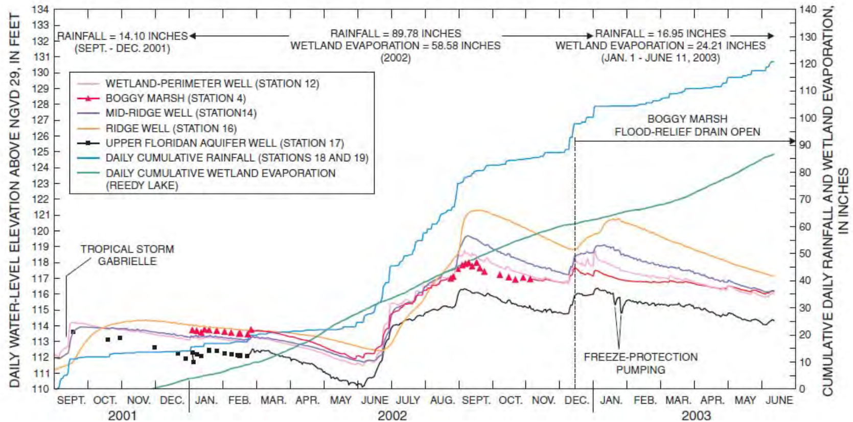
Figure B-17. Figure 19 from Knowles et al. (2005). Original caption reads: “Daily water levels, cumulative rainfall, and cumulative wetland evaporation for the Boggy Marsh site, Hilochee Wildlife Management Area (station numbers refer to figure 5 and table 1).”
